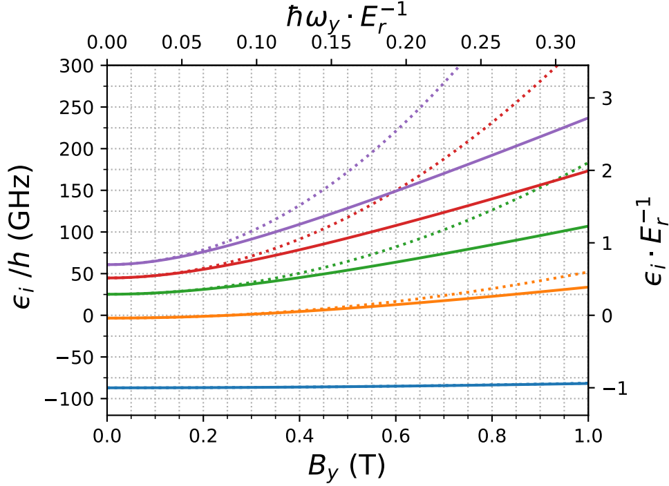
Figure 3.2: Five lowest energy eigenvalues (in GHz) of the Hamiltonian 3.5 for SE on liquid {}^3\text{He} in the perpendicular electric field E_{\perp} = 15 V/cm versus the in-plane magnetic field B_y calculated using the first-order perturbation theory (dashed lines) and numerical solution of the eigenvalue equation (solid lines).
