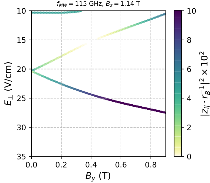
Figure 3.15: Calculated squares of the transition moments for transitions shown in Fig. 3.13. The value of f_{MW} and B_z are adjusted such that the two branches are at resonance when B_y = 0 .
