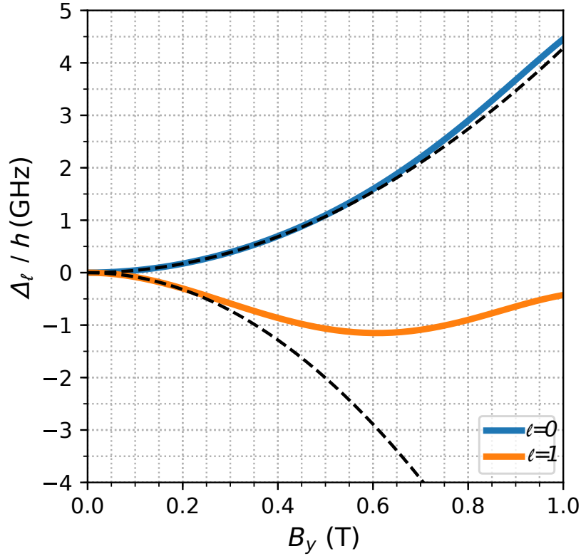
Figure 3.4: The frequency shift of the |1,0\rangle \rightarrow |2,0\rangle transition (blue line) and |1,1\rangle \rightarrow |2,1\rangle transitions (orange line) obtained by the numerical diagonalization of the full Hamiltonian Eq. (3.4) for SE on liquid {}^3\text{He} in the perpendicular magnetic field B_z = 0.65 T and perpendicular electric field E_\perp = 15 V/cm. For the sake of comparison, dashed lines show corresponding shifts obtained from the second order perturbation theory.
