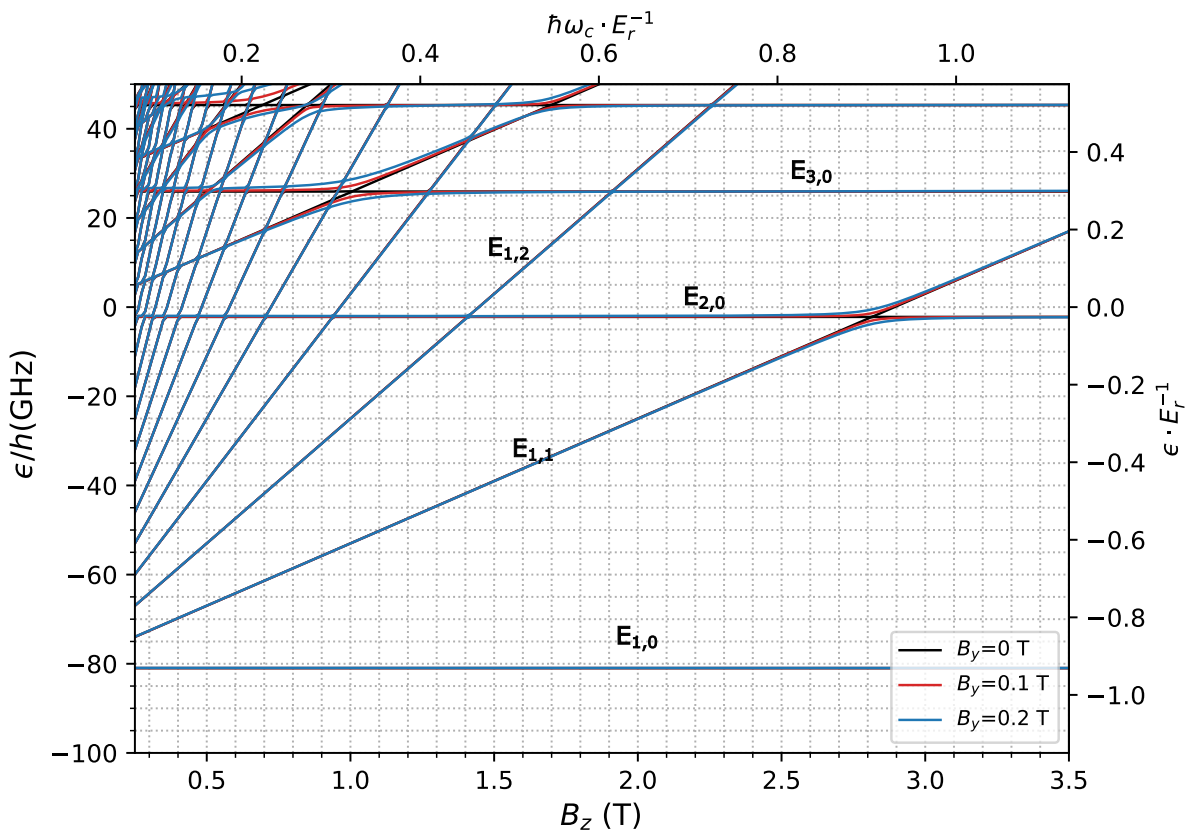
Figure 3.3: Energy eigenvalues (in GHz) of the full Hamiltonian (3.4) for SE on liquid ^3\text{He} in the perpendicular electric field E_\perp = 15 V/cm versus the perpendicular magnetic field B_z . Different colors correspond to the different values of B_y = 0 (black lines), 0.1 (red lines), 0.2 T (blue lines).
