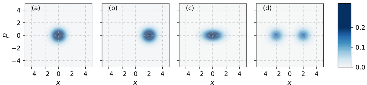
Figure 2.2: The Q-function representation of various pure states |\psi_i\rangle . (a) a vacuum state: |\psi_a\rangle = |0\rangle ; (b) a coherent state: |\psi_b\rangle = D(\alpha = 2) |0\rangle ; (c) a squeezed state |\psi_c\rangle = S(\zeta = -1/2) |0\rangle ; (d) a superposition of two coherent states |\psi_d\rangle = \frac{1}{\sqrt{2}}(D(-2) + D(2)) |0\rangle .
