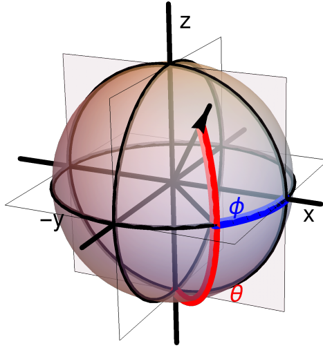
Figure 2.3: Bloch sphere representation of a coherent spin state R(\theta, \phi) |j, -j\rangle .
