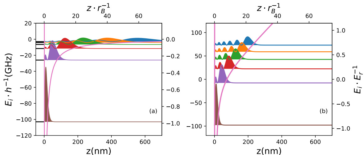
Figure 3.1: Energy eigenvalues (in GHz) and probability densities (in a.u.) for a surface electron on liquid {}^3\text{He} for two values of the perpendicular electric field: E_{\perp} = 0 (a) and E_{\perp} = 15 V/c (b).
