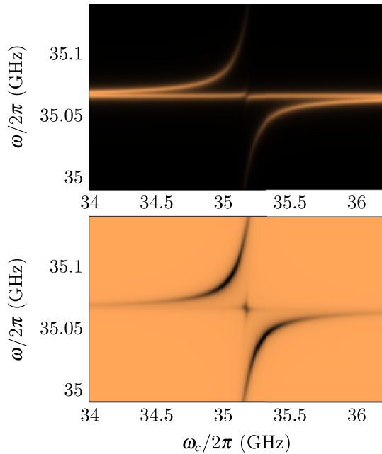
FIG. 7. Power reflection from the cavity (top panel) and power of the Joule heating of 2DES by MW field (bottom panel) versus the cyclotron frequency of electrons \omega_c and the frequency of the MW excitation \omega calculated using the model with the interaction term described by Eq. (26).
