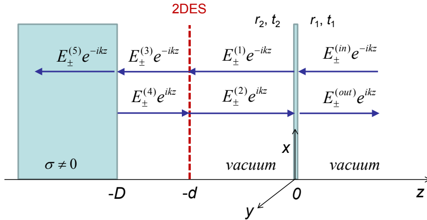
Figure 1.5: Simplified model of the Fabry-Perot resonator containing 2DES as described in the text. Thick arrows (blue) indicate the direction of propagation for different components of EM field inside and outside the resonator excited by the incoming field \mathbf{E}_{in} e^{-i(kz + \omega t)} .
