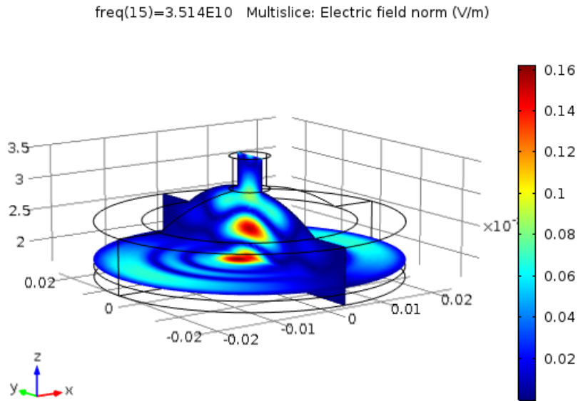
Figure 1.2: COMSOL simulation of the EM mode in a semi-confocal Fabry-Perot microwave (35.14 GHz) cavity resonator.
