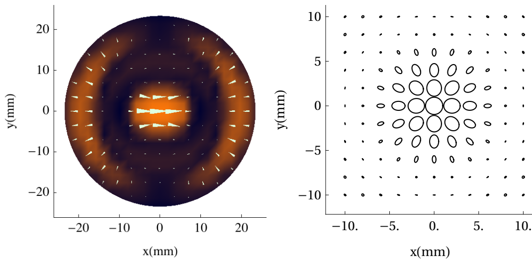
Figure 1.7: (left panel) Distribution of MW electric field on the surface of liquid helium inside the experimental cell under excitation with linearly (x-direction) polarized field. (right panel) Polarization of MW electric field on the surface of liquid helium under excitation with CP field.
