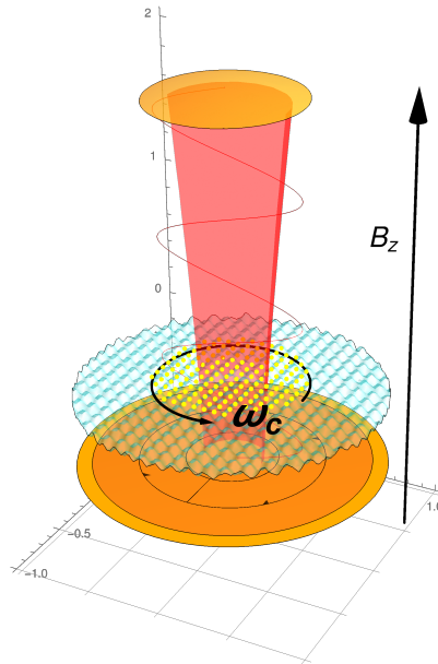
Figure 1.1: An illustration of the experimental setup used to realize the strong coupling between 2D electrons on liquid helium and a single EM mode in an optical resonator.
