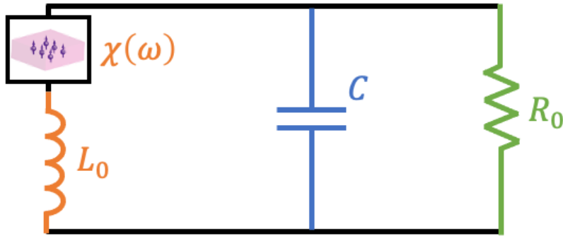
Figure 3.11: The lumped-element representation of the spin-cavity system, with a spin ensemble having susceptibility \chi(\omega) . The real and imaginary parts of the spin susceptibility will modify the total impedance of the system and contribute an additional loss term, respectively. This relationship allows the spin susceptibility to be determined via microwave transmission and reflection measurements.
