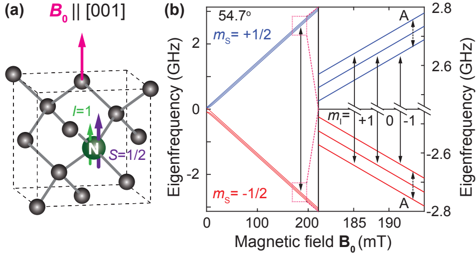
Figure 4.8: The P1 center in the [001] B-field orientation. a) The P1 centers are uniformly aligned to an angle of 54.7^\circ along the static field, meaning that it is possible to drive all spins together with an AC microwave field. b) Energy levels of the m_s = -1/2, 1/2 spin sublevels of P1 for the [001] B-field orientation. Zooming in on the region around 185 mT reveals three hyperfine transitions ( m_i = -1, 0, \text{ and } +1 ), which are well-resolved due to the relatively large hyperfine tensor ( |A| \approx 94 MHz). The point where each of the three hyperfine transitions reaches 5.295 GHz is labeled with a black arrowed line.
