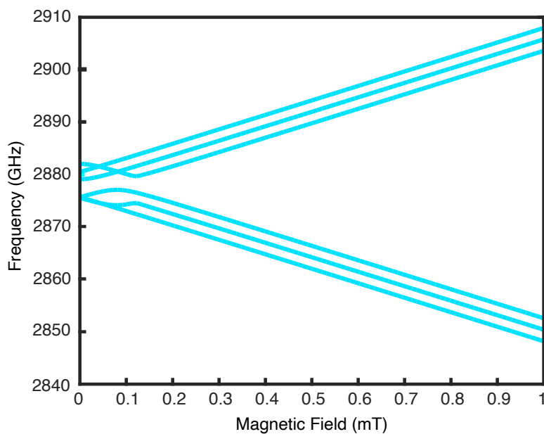
Figure 1.5: The hyperfine levels of an NV center at low field, showing splitting of Assuming the nuclear spin is conserved, this creates three possible transitions between each level.
