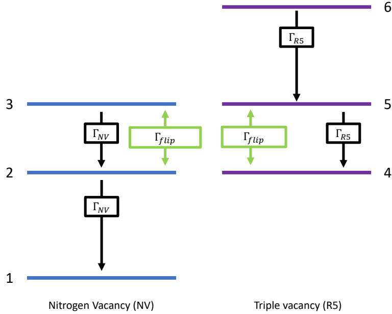
Figure 5.5: The spin flip-flop interaction model for NV/R5. The three spin states of NV (R5) are labeled 1-3 (4-6). The B-field has been tuned in such a way that the transition NV_{2-3} is co-resonant with the transition R5_{4-5} . Energy is exchanged between these four levels at the rate \Gamma_{flip} . In addition, spins in each upper level relax to the lower levels at the rates \Gamma_{NV} and \Gamma_{R5} , respectively. If there is a large asymmetry in the relaxation rates, a population inversion should manifest on the transition NV_{1-2} .
